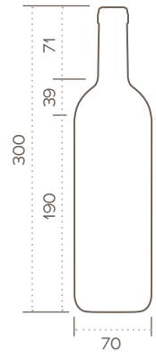
Standard Bordeaux style bottle dimensions
